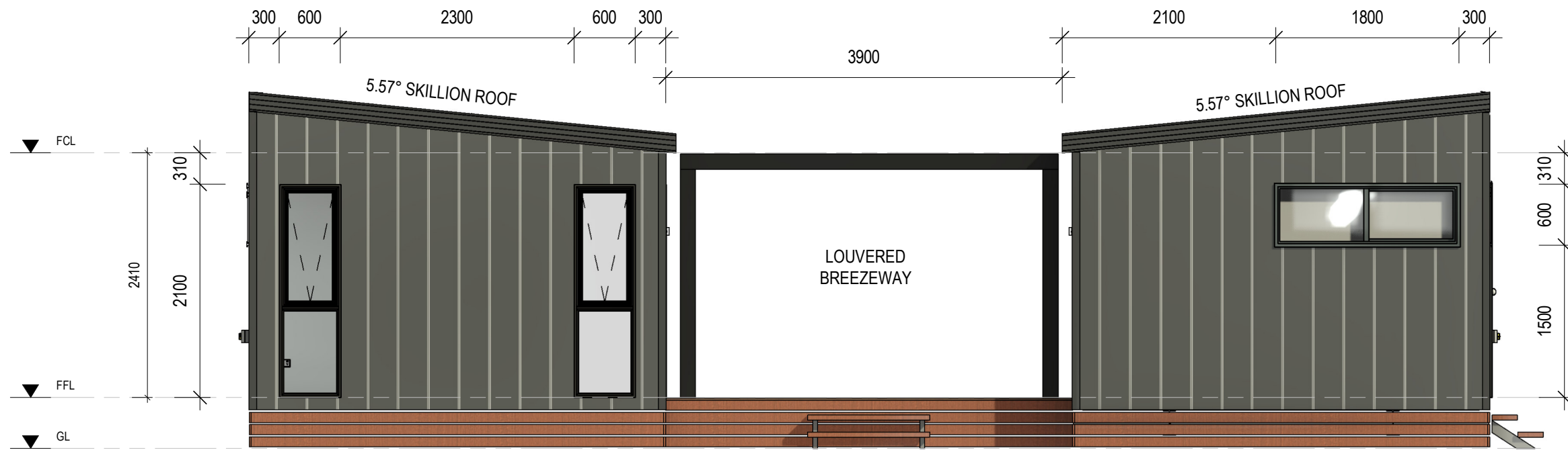
3 RIGHT ELEVATION (3) A103 1 : 50
